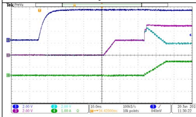
Figure 6. Soft Start into Cooling Mode ( V_{IN}=5\text{V} with 2\Omega load)
