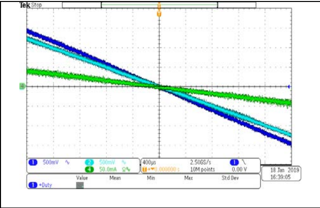
Figure 10. Zero Crossing TEC Current Zoom-in from Cooling to Heating (Line 1: LDR (TEC+), Line 2: SFB (TEC-), Line 4: ITEC)
