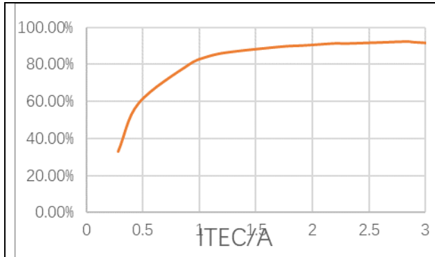
Figure 4. Efficiency vs. ITEC at V_{IN}=5.0\text{V} With 1\Omega Load in Cooling Mode
