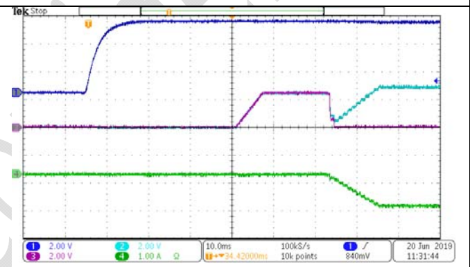
Figure 7. Soft Start into Heating Mode ( V_{IN}=5.0\text{V} with 2\Omega load)
