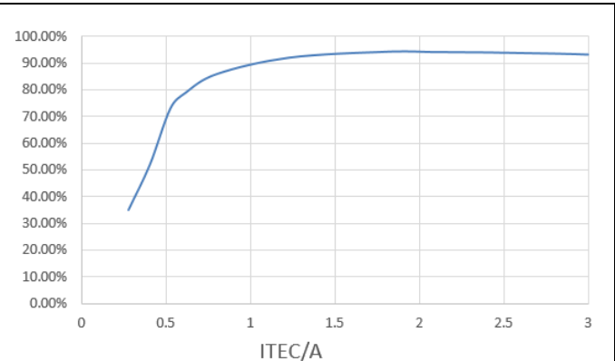
Figure 5. Efficiency vs. ITEC at V_{IN}=5.0\text{V} With 1\Omega Load in Heating Mode
